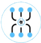
TESTING ALGORITHM
